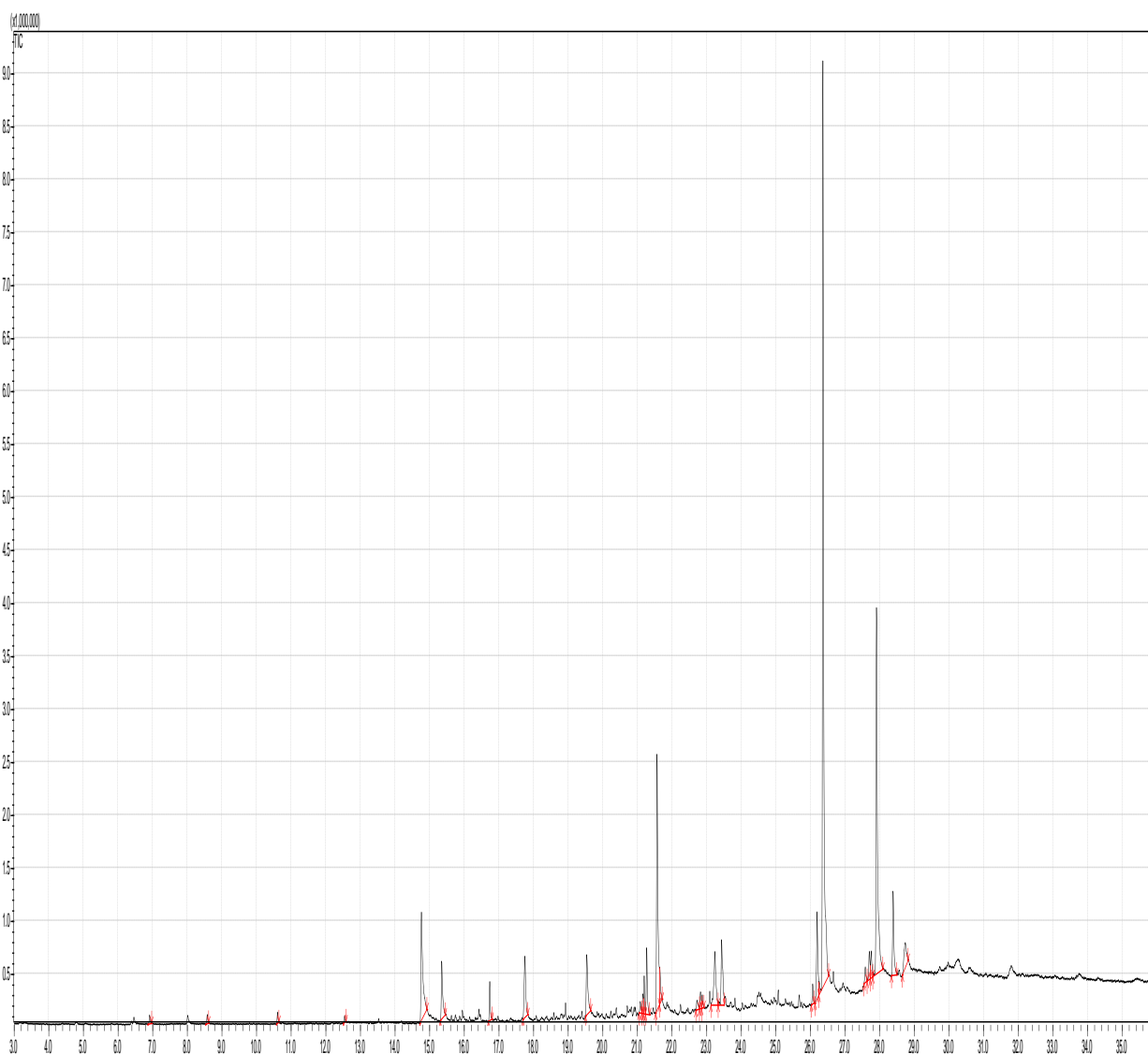
Fig. 2: GC-MS Chromatogram of Bryum coronatum Schwager.
