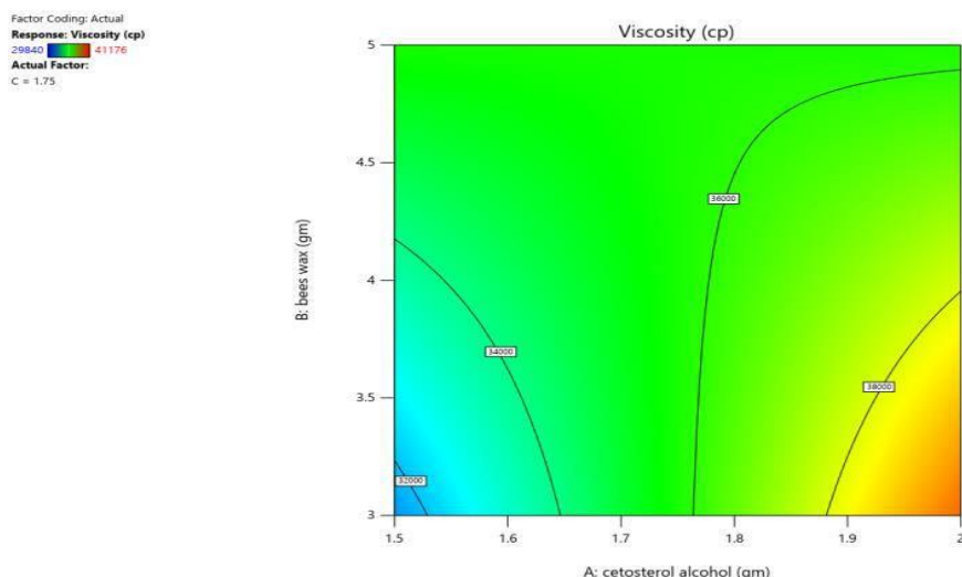
Figure 4: Contour Plot Showing the Influence of Viscosity.
