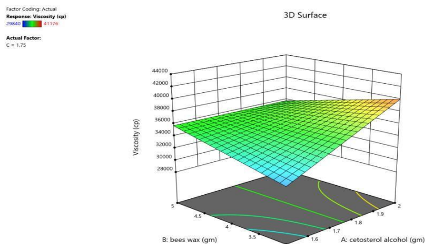
Figure 5. Response Surface Plot Showing the Viscosity.
