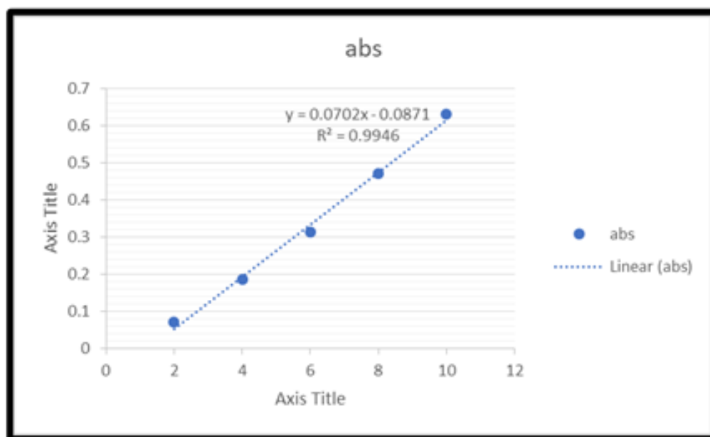
Figure 1: Calibration Curve of Curcumin Standard Solution.
