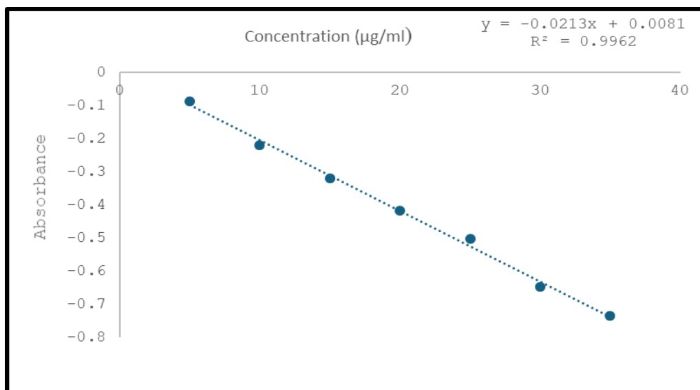
Figure 4: Calibration Curve of DXL at 293.20 nm.
