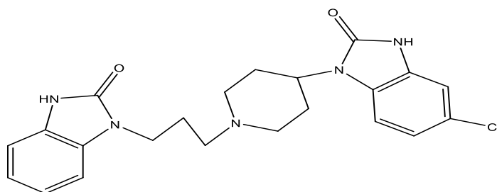
Domperidone
